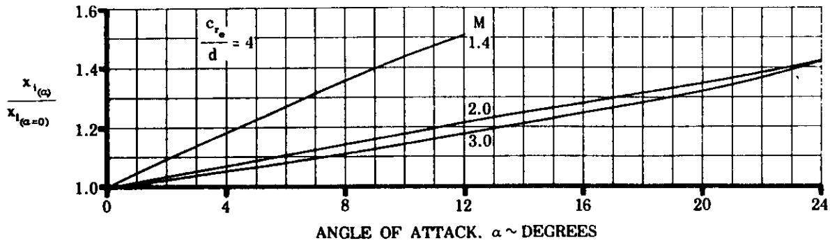
FIGURE 5.2.3.2-6 EFFECT OF ANGLE OF ATTACK ON CENTER-OF-PRESSURE LOCATION OF WING-INDUCED BODY SIDE FORCE
