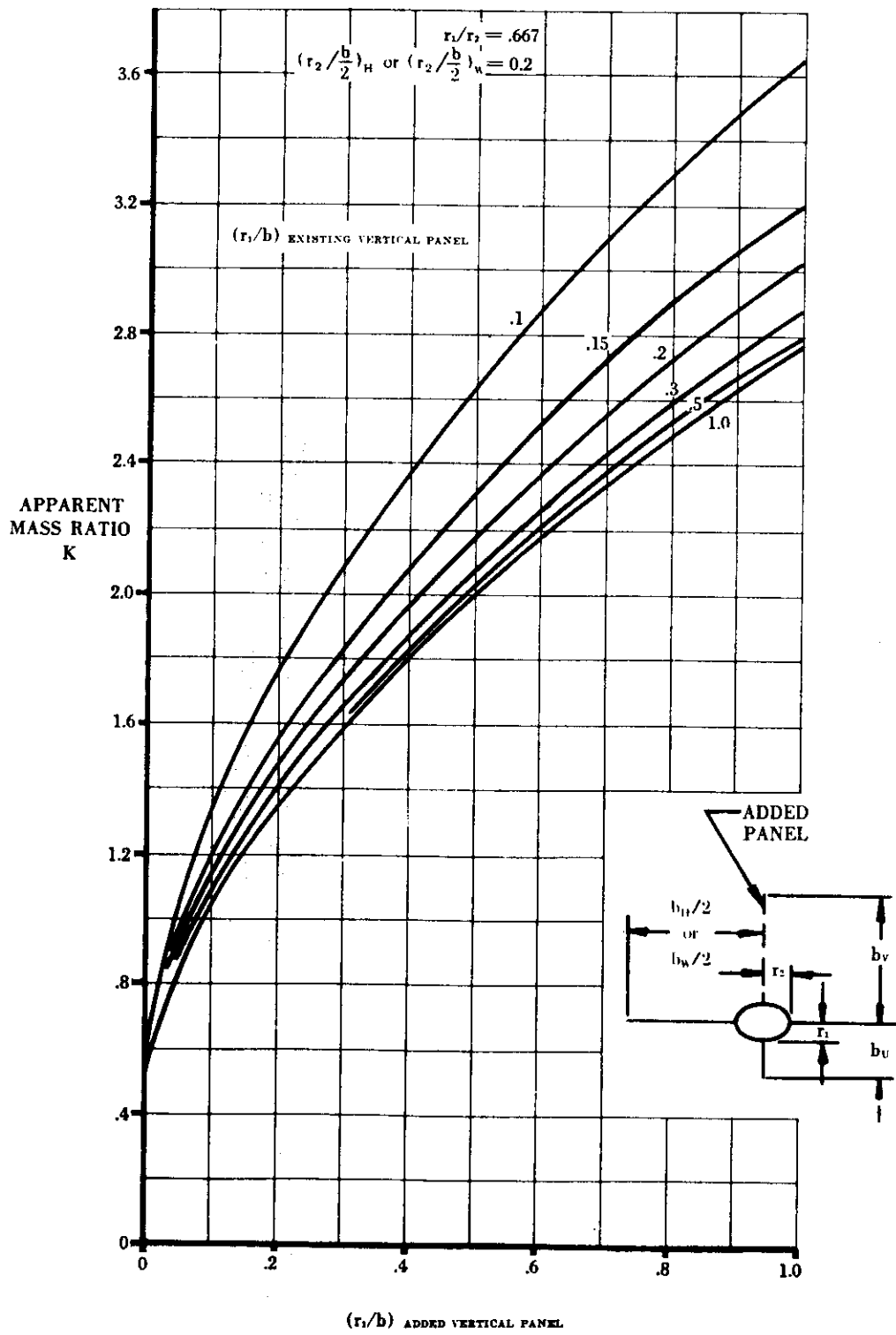
FIGURE 5.3.1.1-25y APPARENT MASS FACTORS (CONTD)
