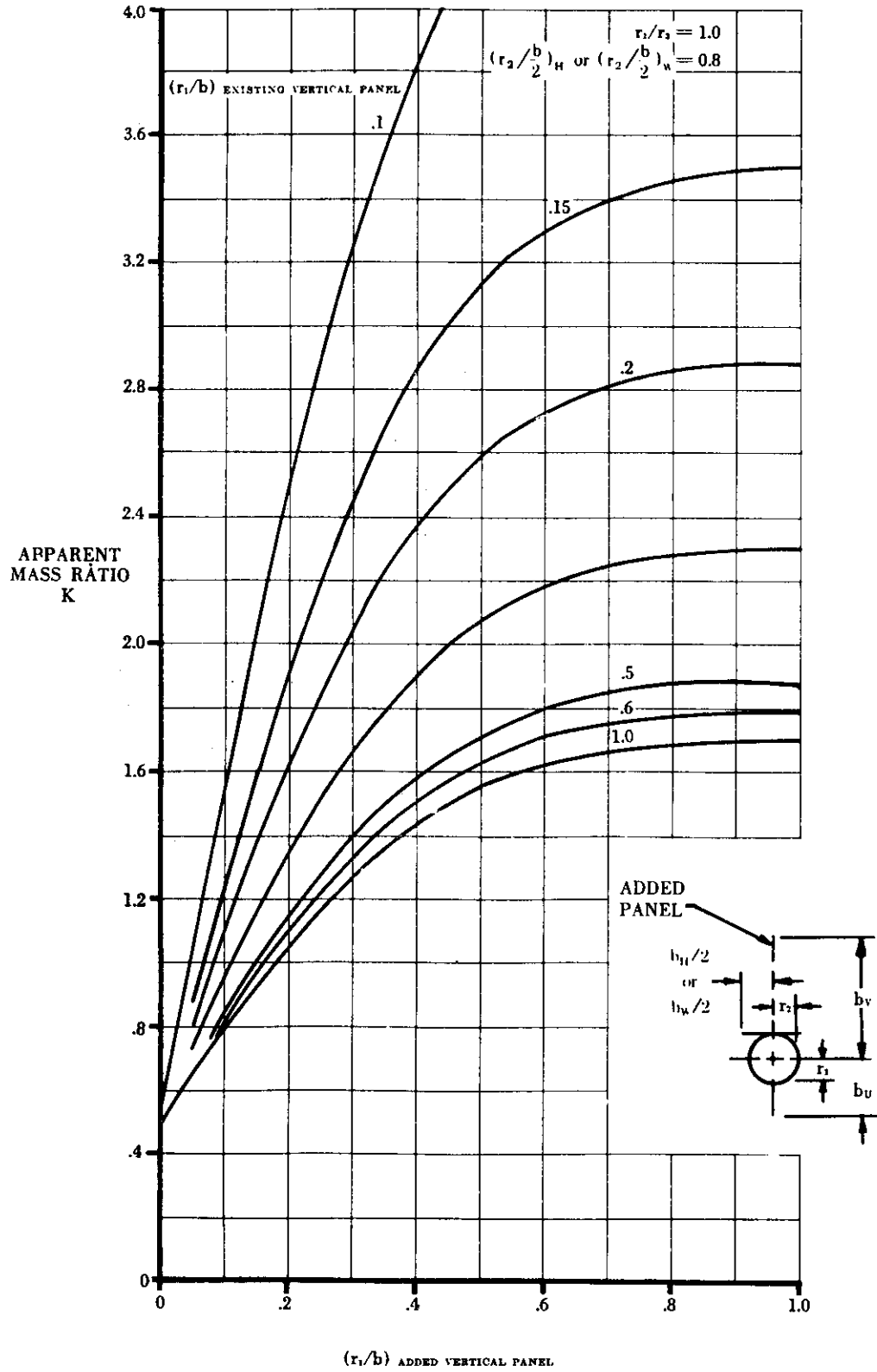
FIGURE 5.3.1.1-25k APPARENT MASS FACTORS (CONTD)
