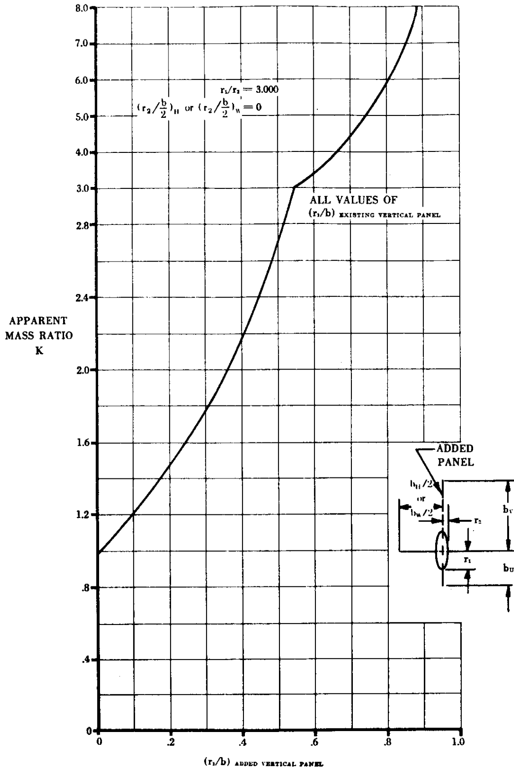
FIGURE 5.3.1.1-25j APPARENT MASS FACTORS (CONTD)
