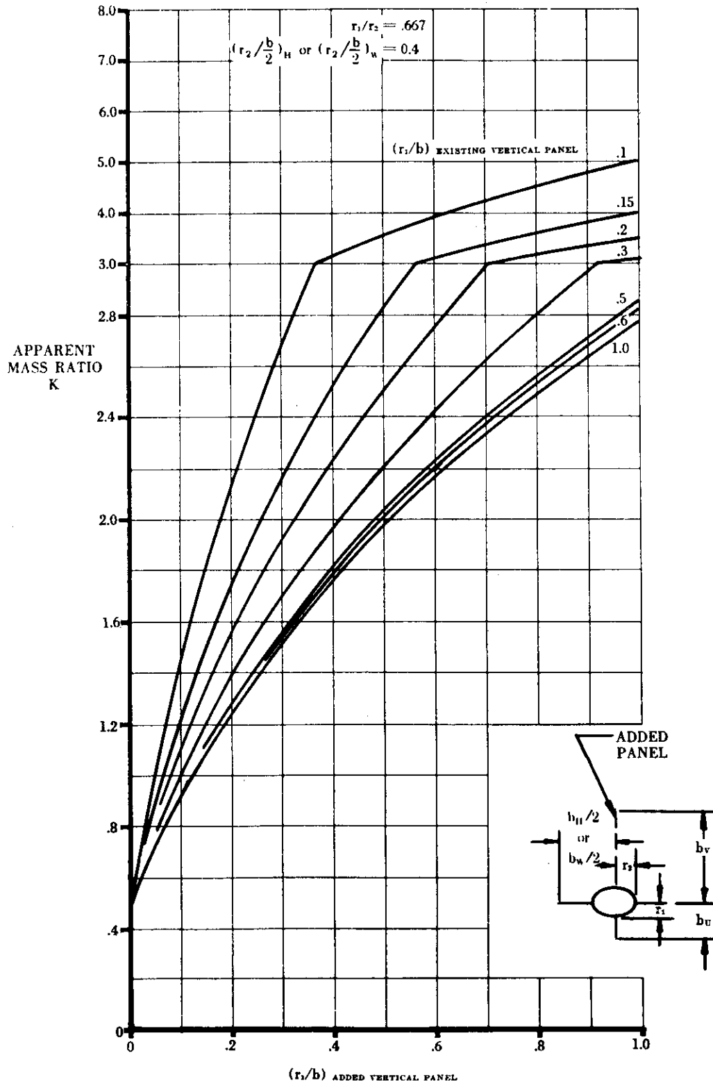
FIGURE 5.3.1.1-25z APPARENT MASS FACTORS (CONTD)
