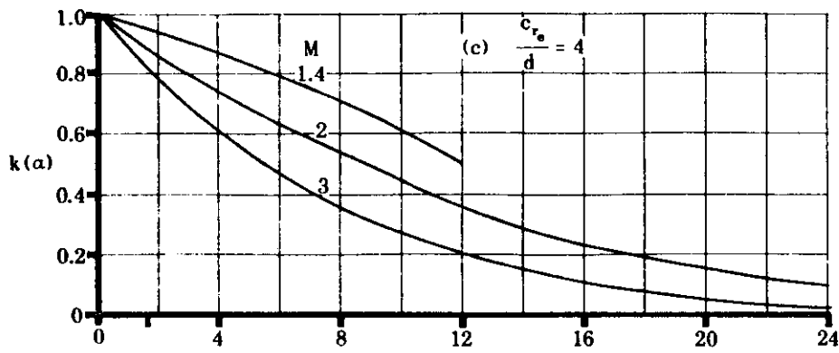
FIGURE 5.2.1.2-8 ANGLE-OF-ATTACK CORRECTION TO WING-BODY INTERFERENCE COEFFICIENT
