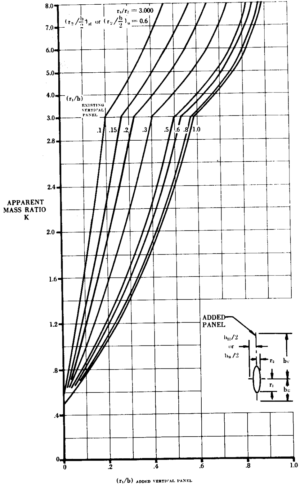
FIGURE 5.3.1.1-25mm APPARENT MASS FACTORS (CONTD)
