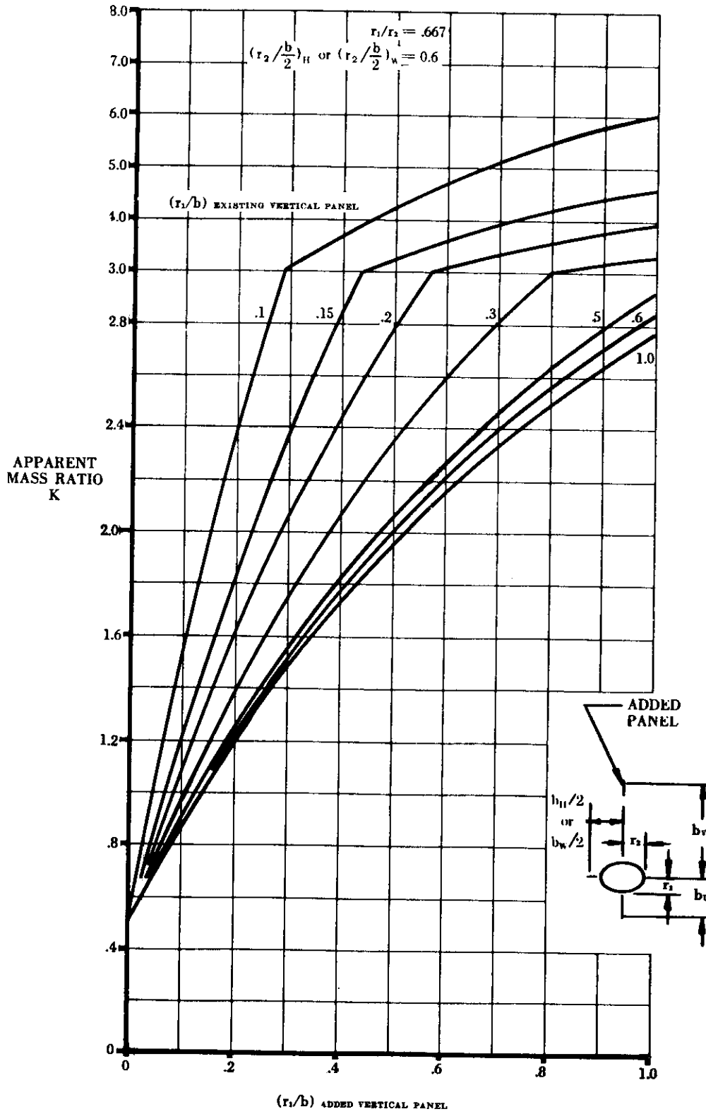
FIGURE 5.3.1.1-25aa APPARENT MASS FACTORS (CONTD)
