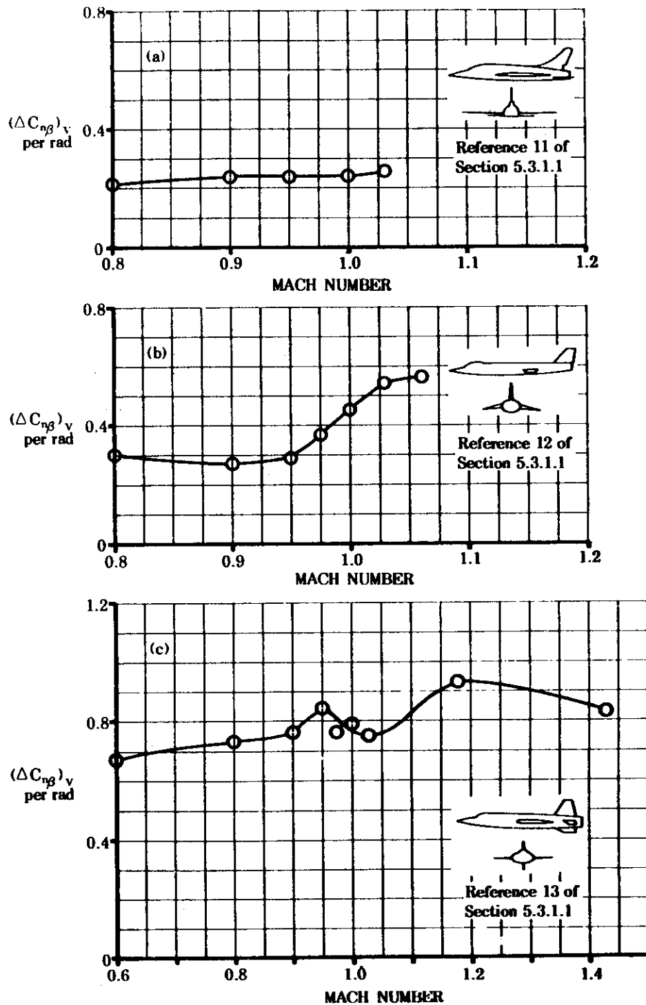
FIGURE 5.3.3.1-11. TYPICAL TRANSONIC DATA
