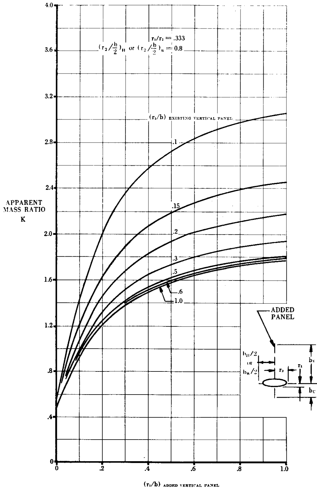
FIGURE 5.3.1.1-25v APPARENT MASS FACTORS (CONTD)
