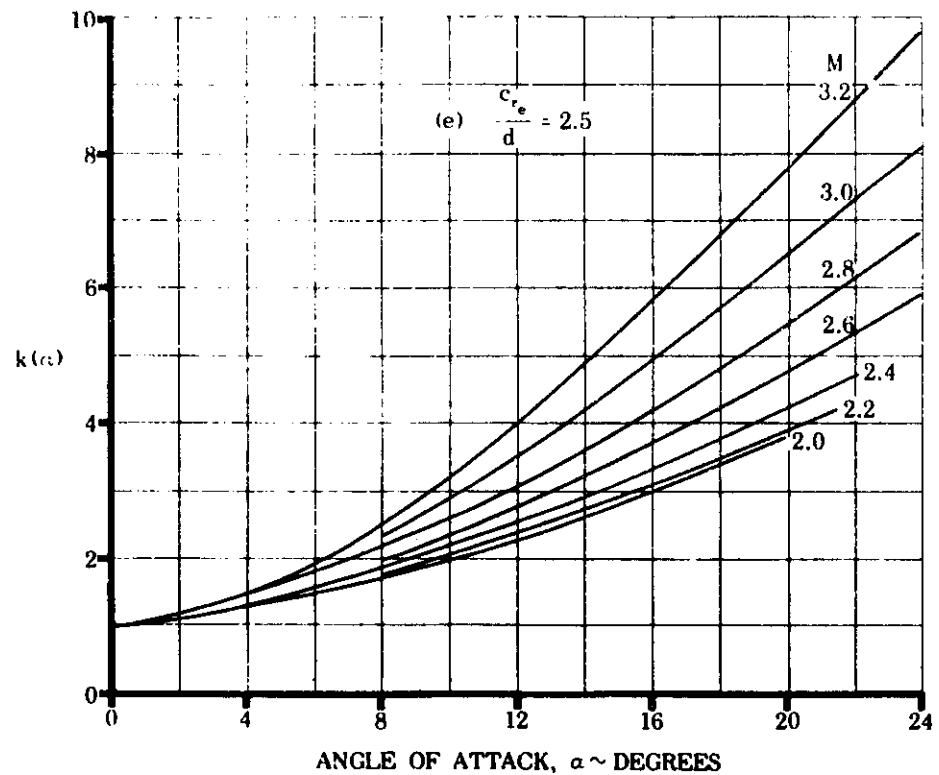
FIGURE 5.2.1.2-8 ANGLE-OF-ATTACK CORRECTION TO WING-BODY INTERFERENCE COEFFICIENT (contd)
