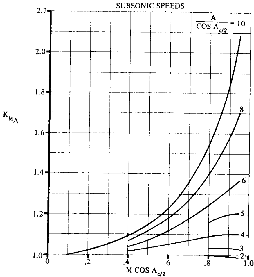
FIGURE 5.1.2.1-28a COMPRESSIBILITY CORRECTION FACTOR TO SWEEP CONTRIBUTION TO WING C_{l\beta}
