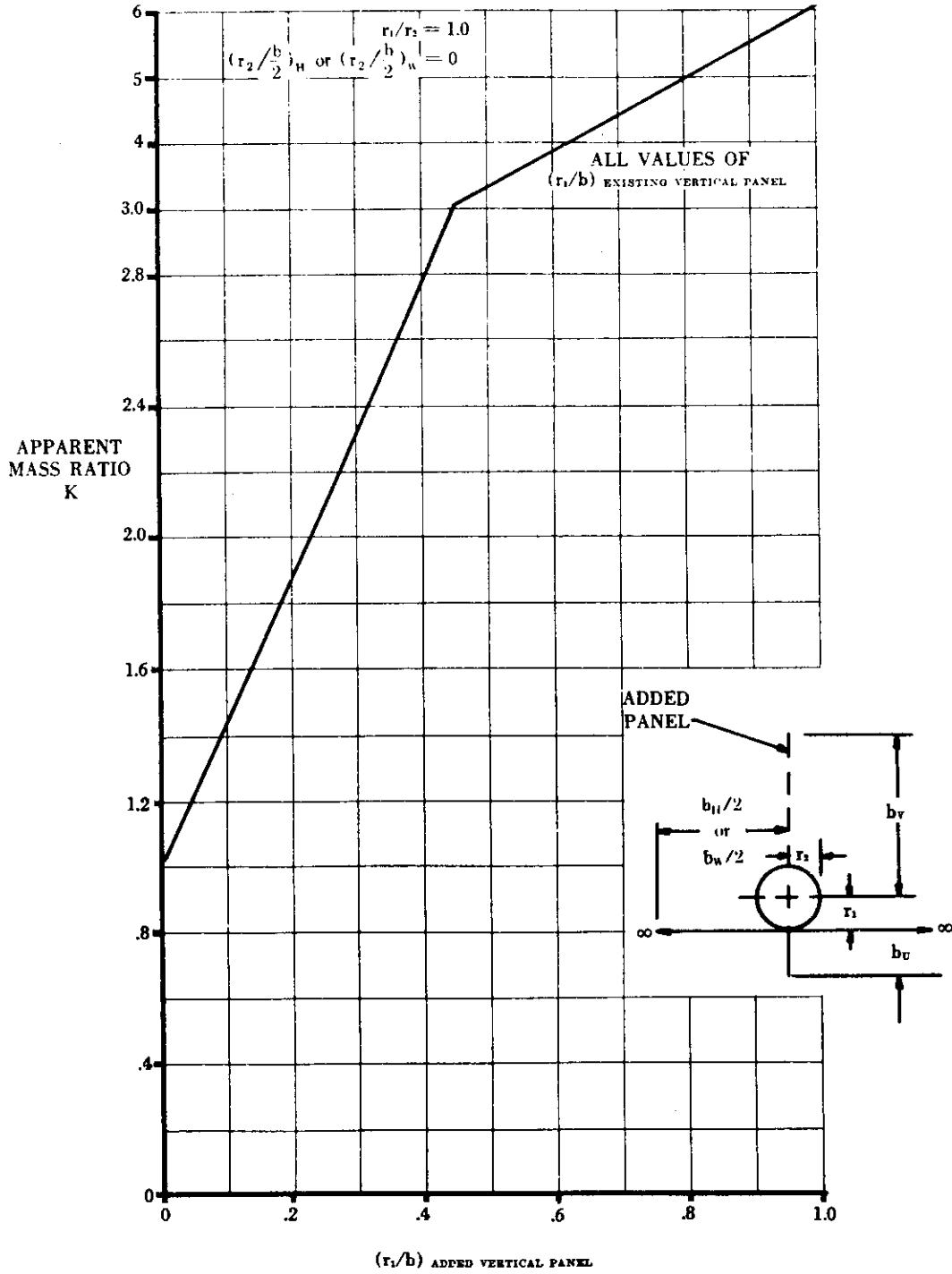
FIGURE 5.3.1.1-251 APPARENT MASS FACTORS (CONTD)
