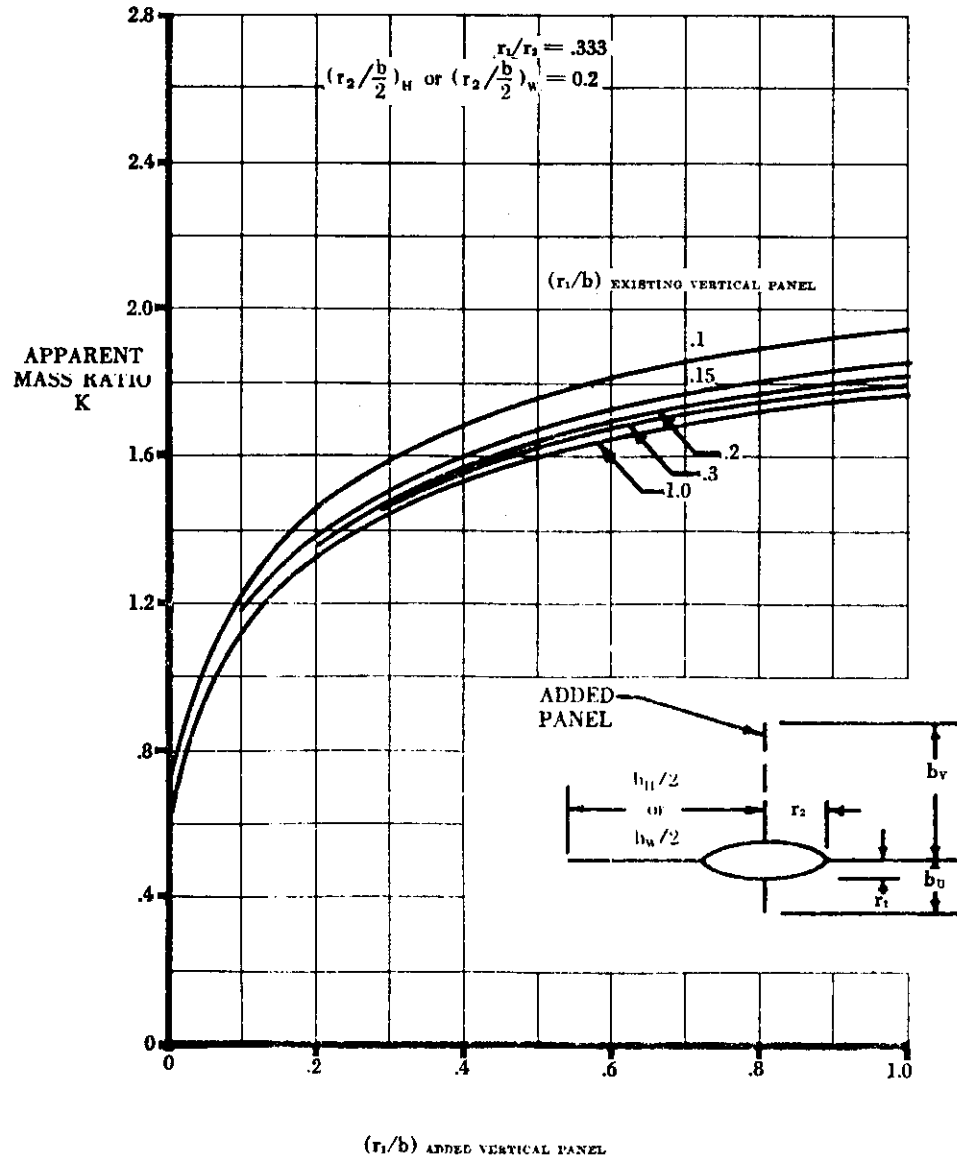
FIGURE 5 1.1.1-25: APPARENT MASS FACTORS (CONTD)
