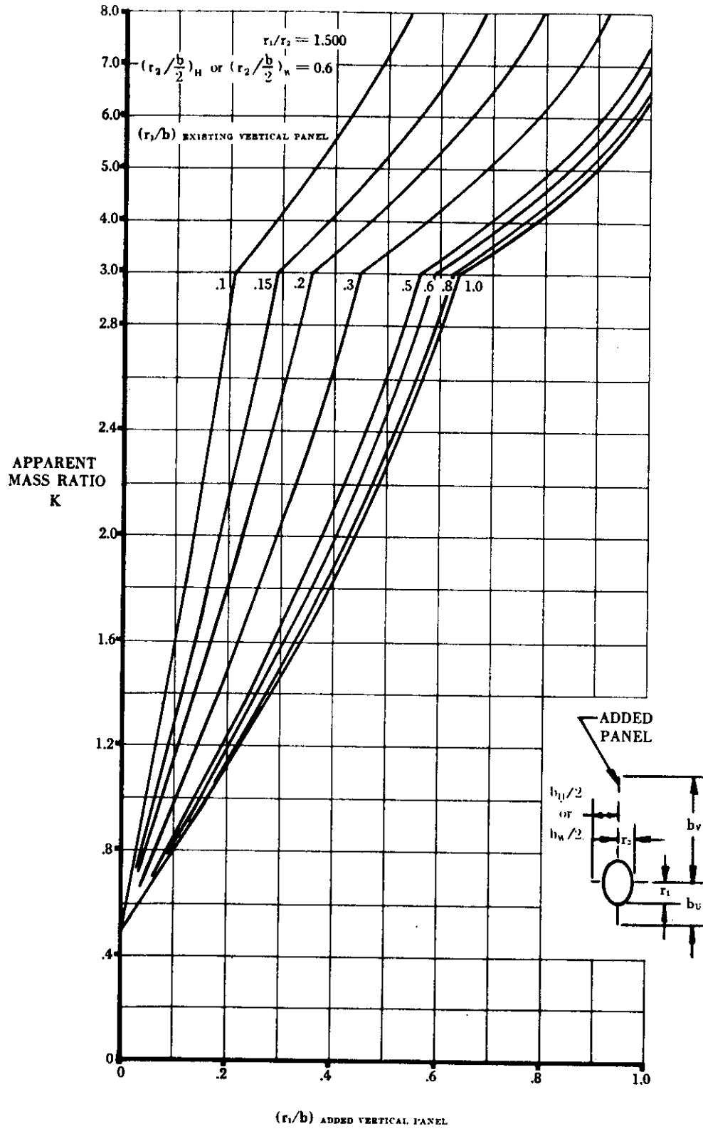
FIGURE 5.3.1.1-25g APPARENT MASS FACTORS (CONTD)
