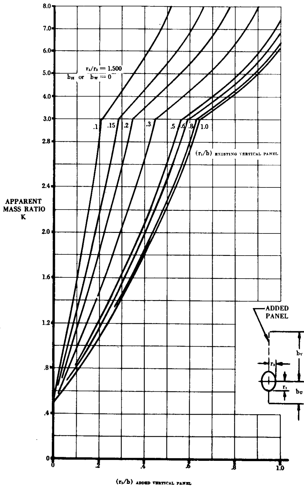
FIGURE 5.3.1.1-25cc APPARENT MASS FACTORS (CONTD)
