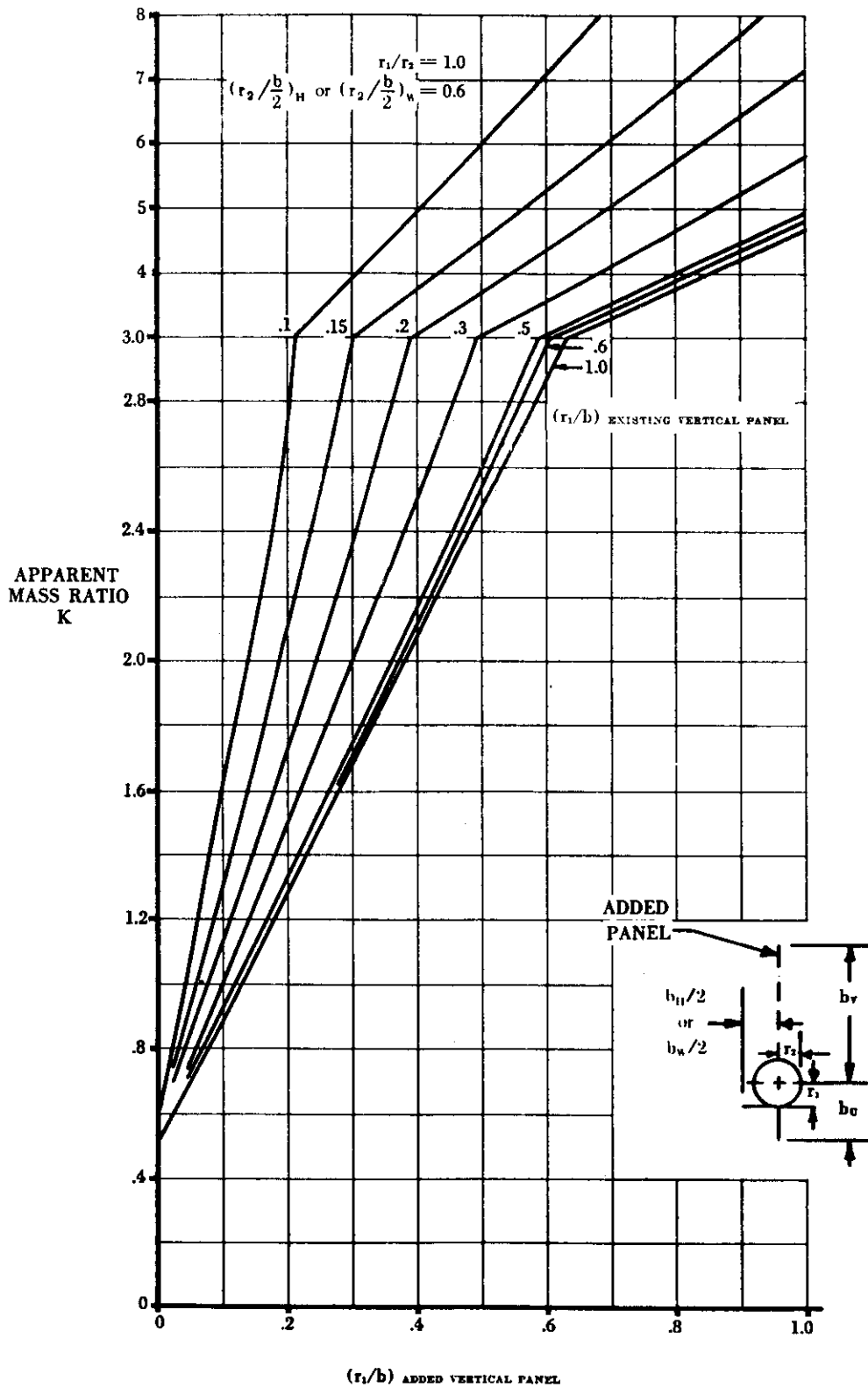
FIGURE 5.3.1.1-250 APPARENT MASS FACTORS (CONTD)
