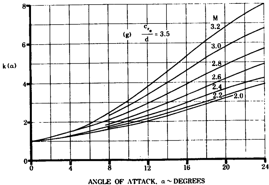
ANGLE OF ATTACK, \alpha \sim DEGREES FIGURE 5.2.1.2-8 ANGLE-OF-ATTACK CORRECTION TO WING-BODY INTERFERENCE COEFFICIENT (contd)
