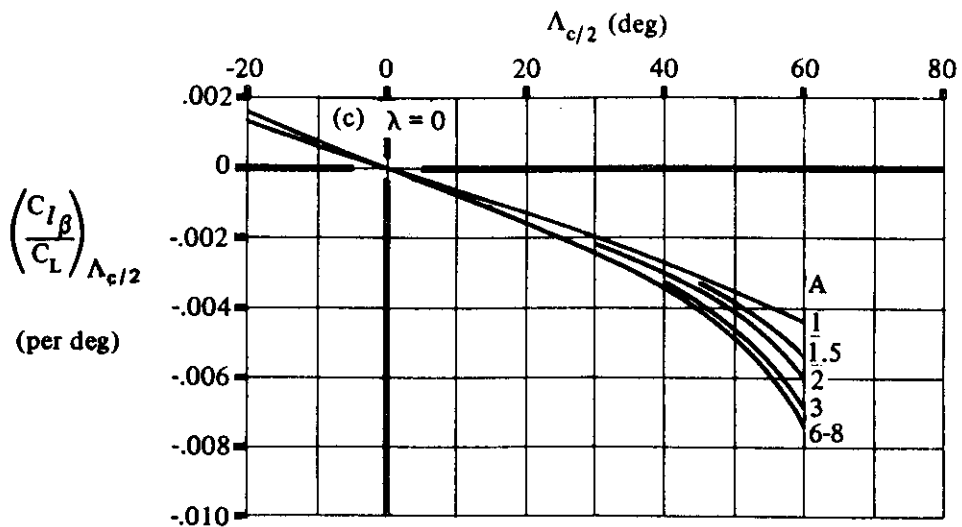
FIGURE 5.1.2.1-27 WING SWEEP CONTRIBUTION TO C_{l\beta}
