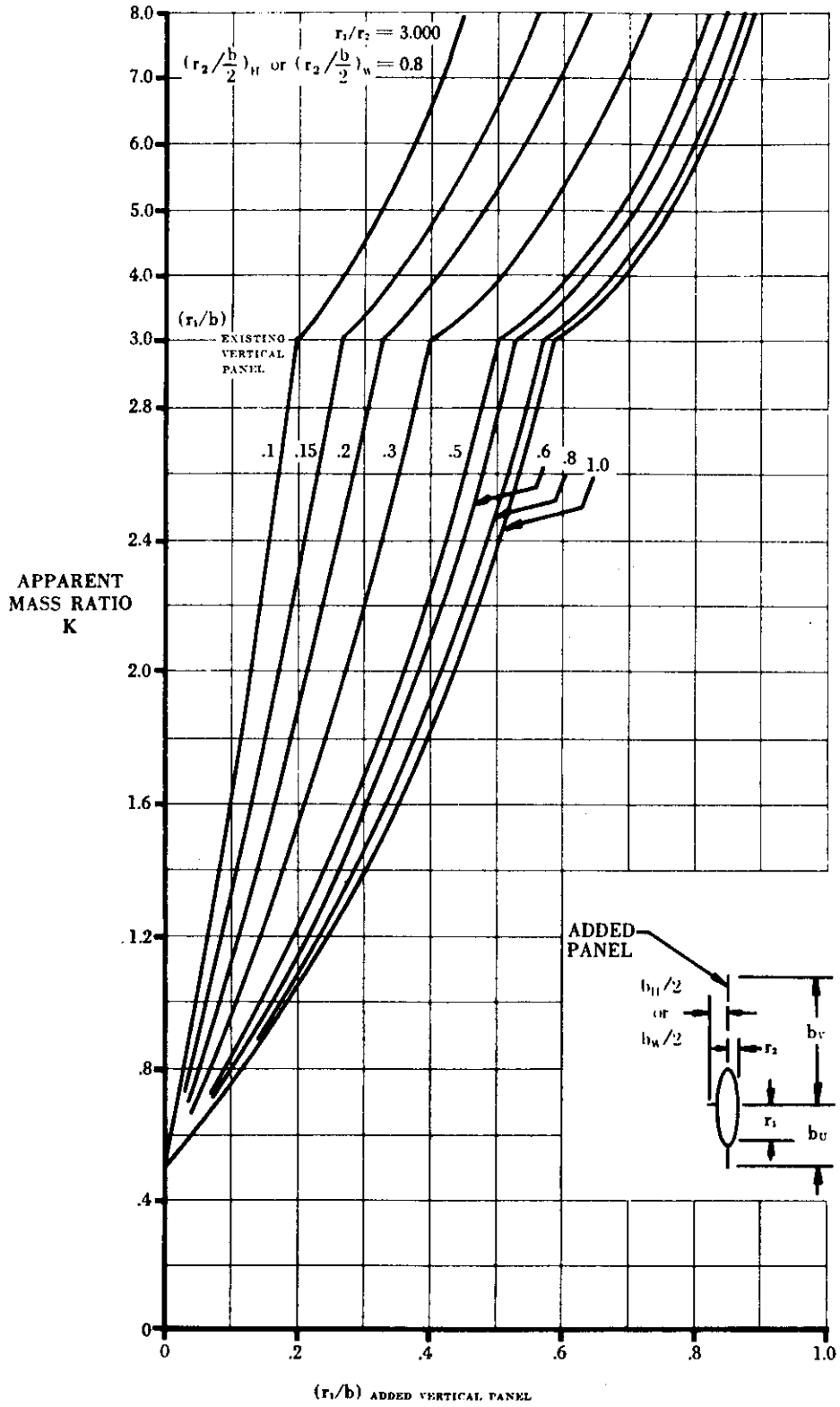
FIGURE 5.3.1.1-25nn APPARENT MASS FACTORS (CONTD)
