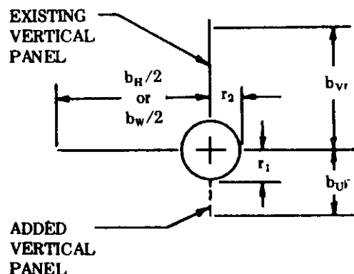
SKETCH (a)
