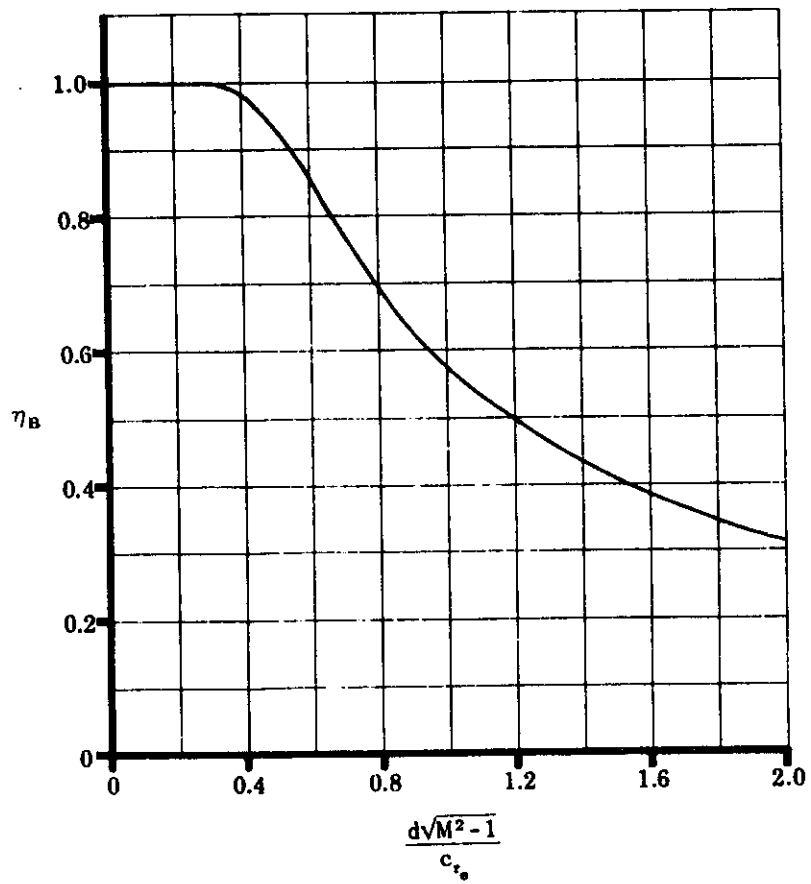
FIGURE 5.2.1.2-7 MACH NUMBER CORRECTION TO WING-BODY INTERFERENCE COEFFICIENT
