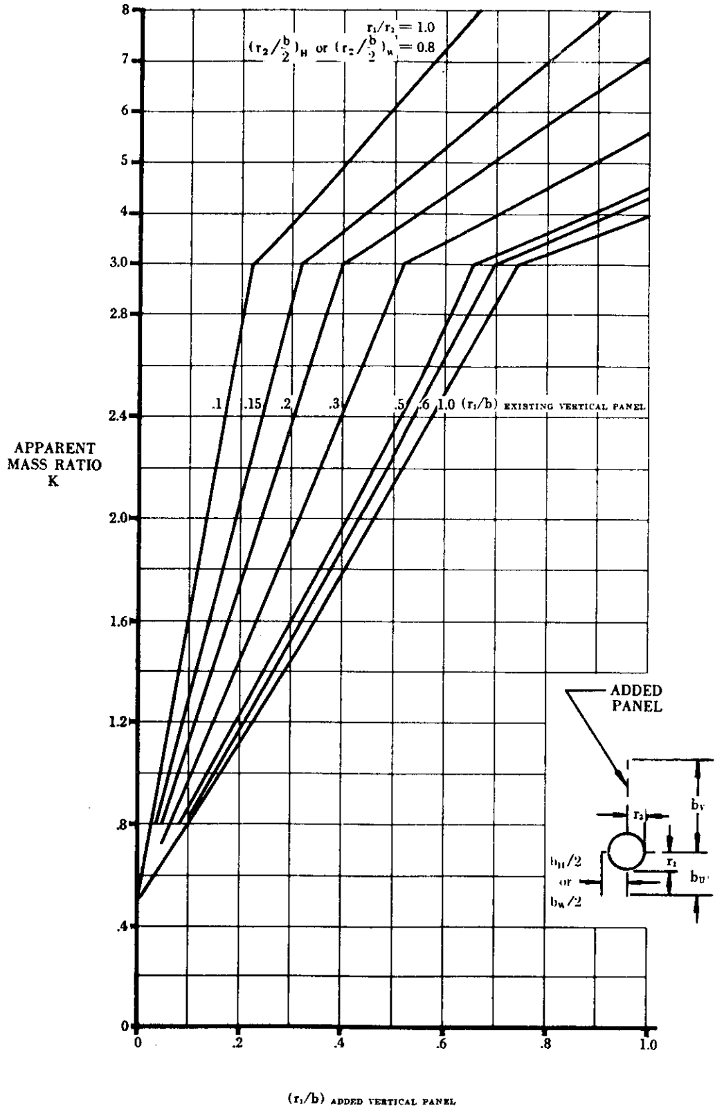
FIGURE 5.3.1.1-25f APPARENT MASS FACTORS (CONTD)
