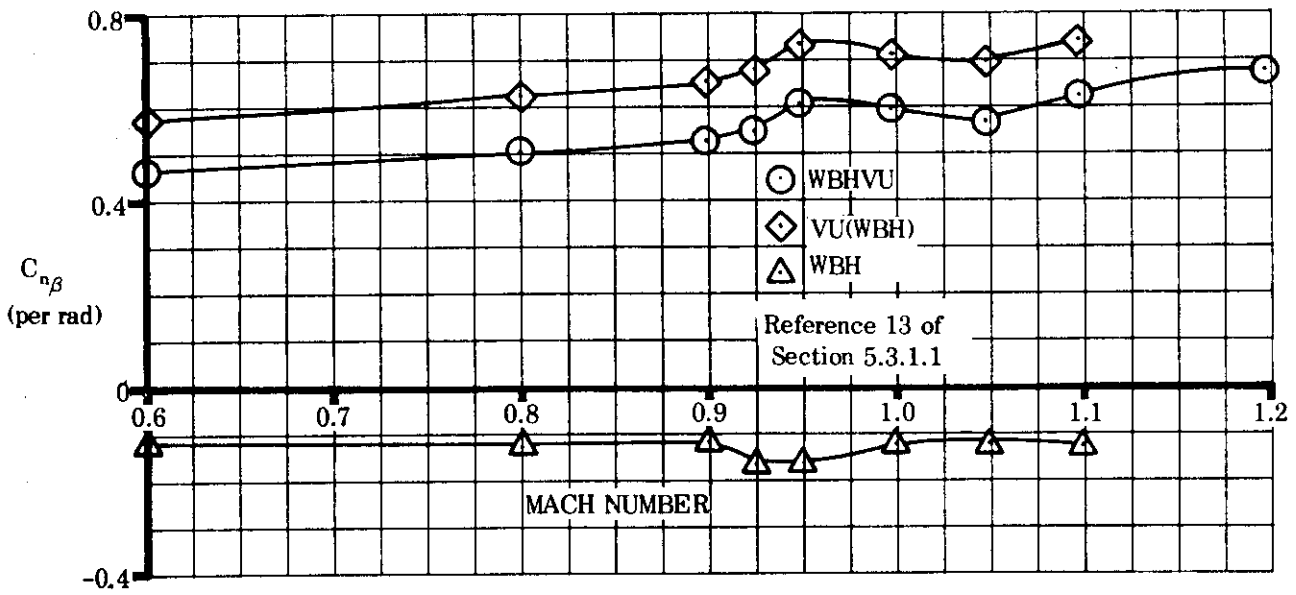
FIGURE 5.6.3.1-8 TYPICAL TRANSONIC DATA
