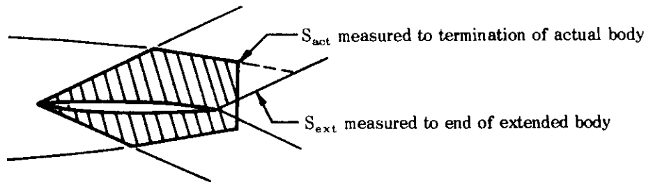
SKETCH (c)
