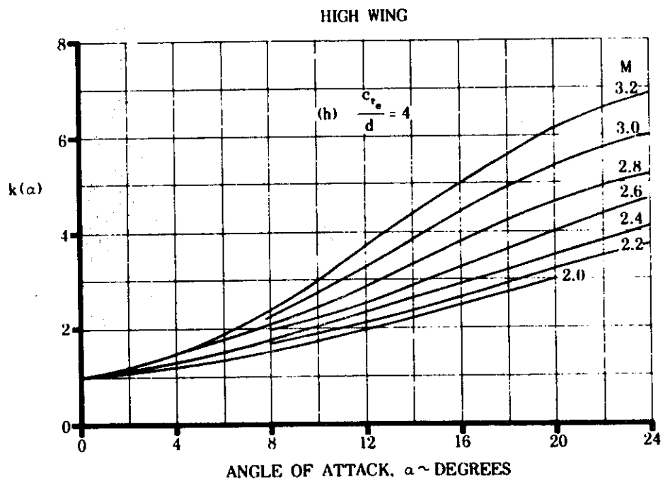
FIGURE 5.2.1.2-8 ANGLE-OF-ATTACK CORRECTION TO WING-BODY INTERFERENCE COEFFICIENT (contd)
