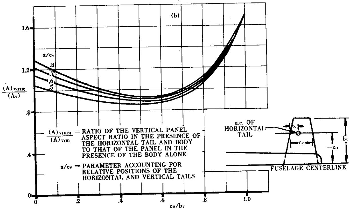
FIGURE 5.3.1.1-22 CHARTS FOR ESTIMATING THE SIDESLIP DERIVATIVE (C_{Yp})_{v(WBH)} FOR SINGLE VERTICAL TAILS
