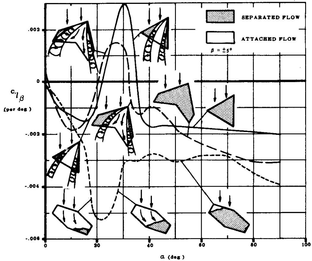
FIGURE 5.1.2.2-4 EFFECT OF PLANFORM ON THE VARIATION OF C_{l\beta} WITH ANGLE OF ATTACK, ZERO DIHEDRAL, LOW SPEEDS (FROM REF. 1).
