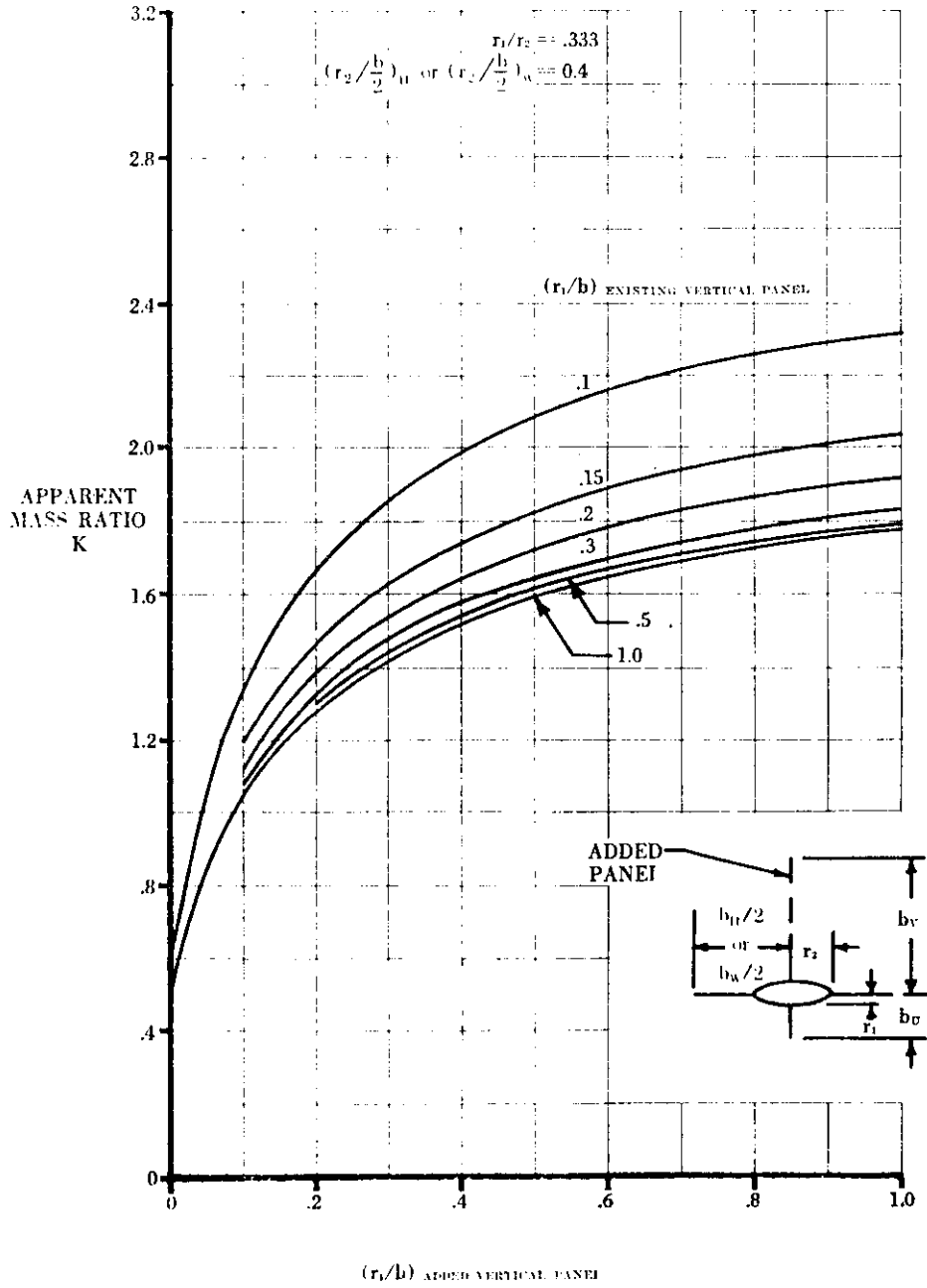
FIGURE 5.3.1.1-25t APPARENT MASS FACTORS (CONTD)
