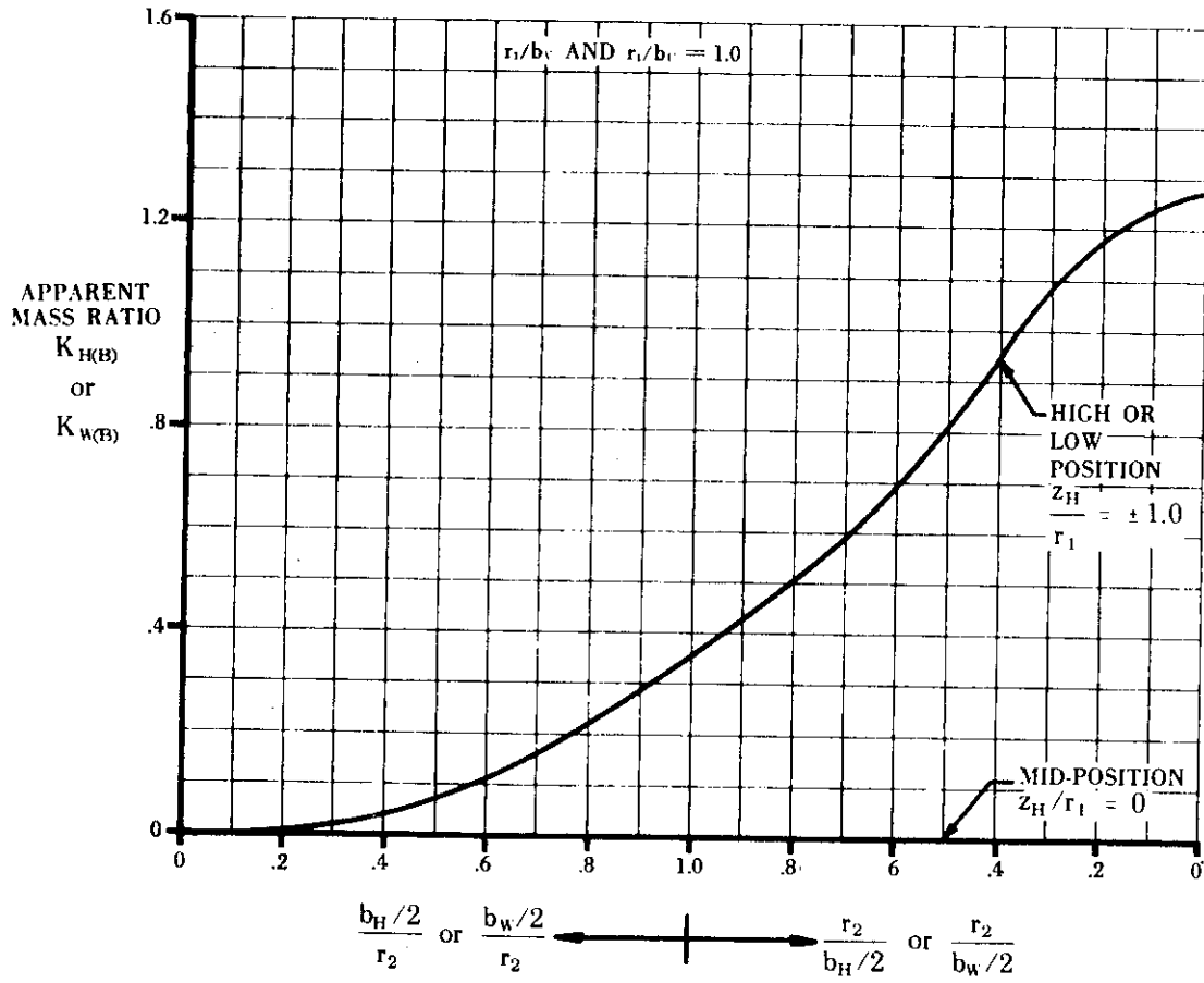
FIGURE 5.3.1.1-2500 APPARENT MASS FACTORS (CONTD)
