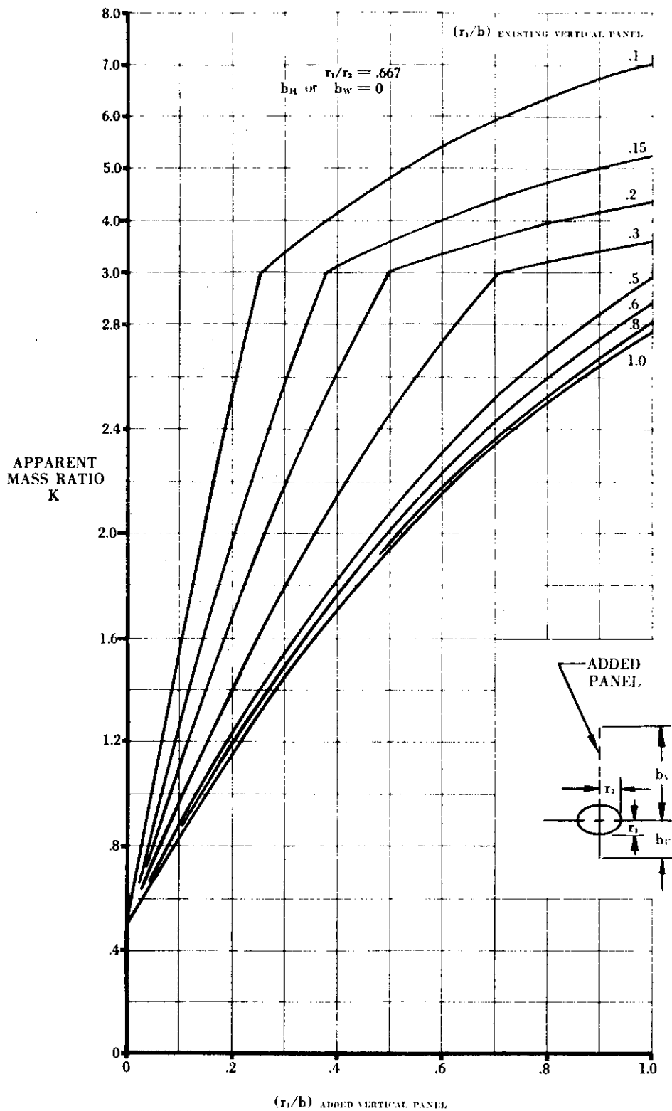
FIGURE 5.3.1.1-25w APPARENT MASS FACTORS (CONTD)
