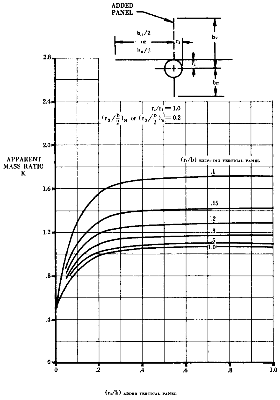
FIGURE 5.3.1.1-25h APPARENT MASS FACTORS (CONTD)
