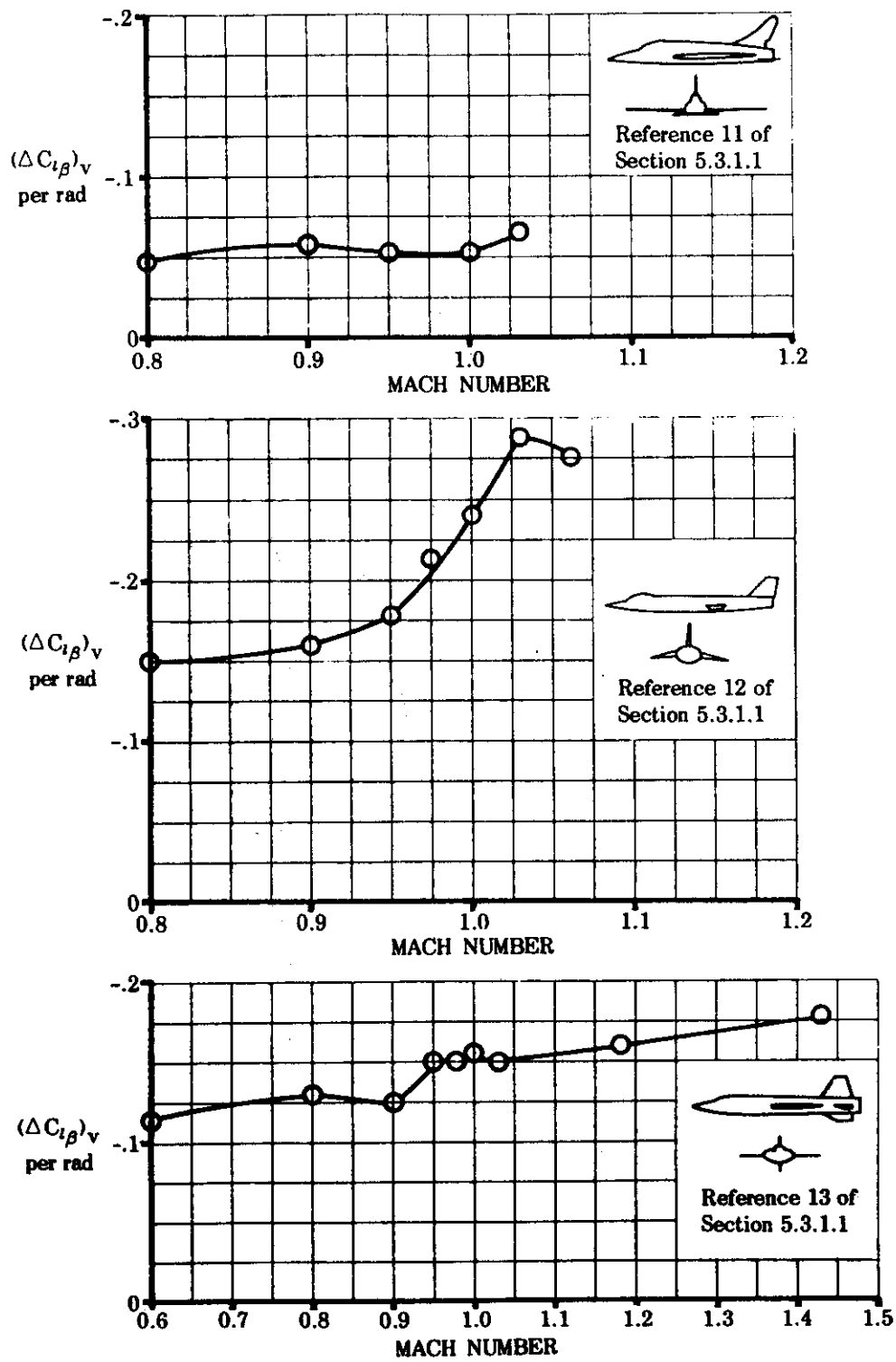
FIGURE 5.3.2.1-13 TYPICAL TRANSONIC DATA
