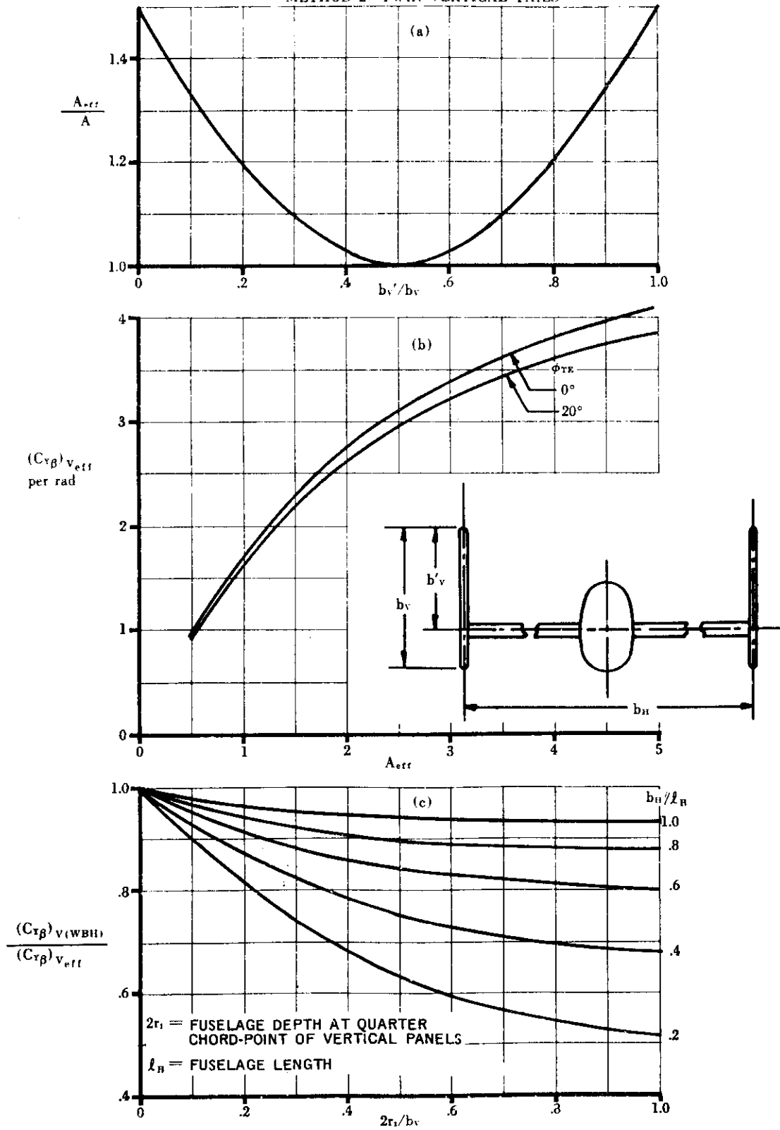
FIGURE 5.3.1.1-24 CHARTS FOR ESTIMATING THE SIDESLIP DERIVATIVE (C_{Y\beta})_{V(WBH)} FOR TWIN VERTICAL TAILS.
