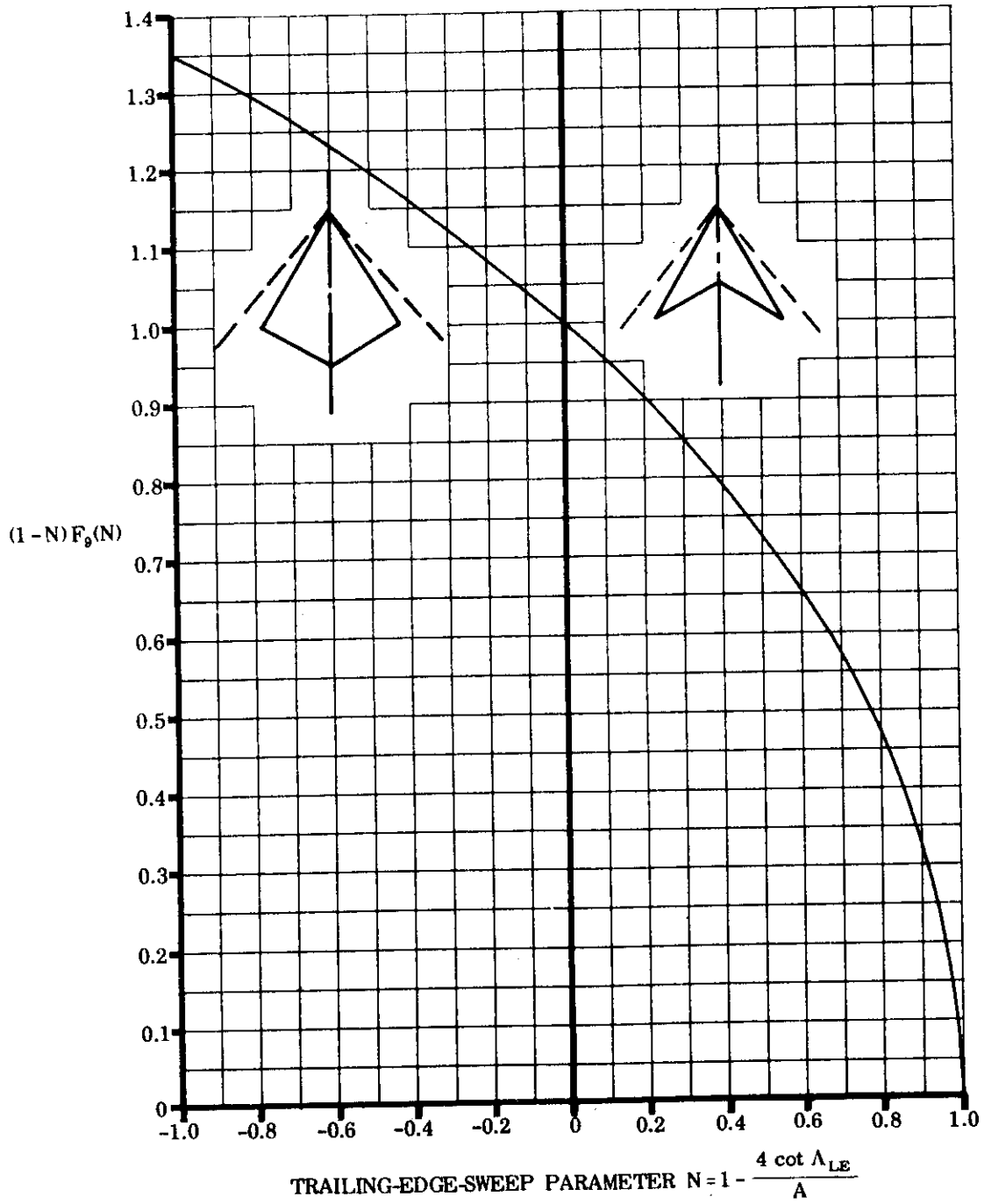
FIGURE 5.1.3.1-6 F_9(N) FACTOR OF THE STABILITY DERIVATIVE
