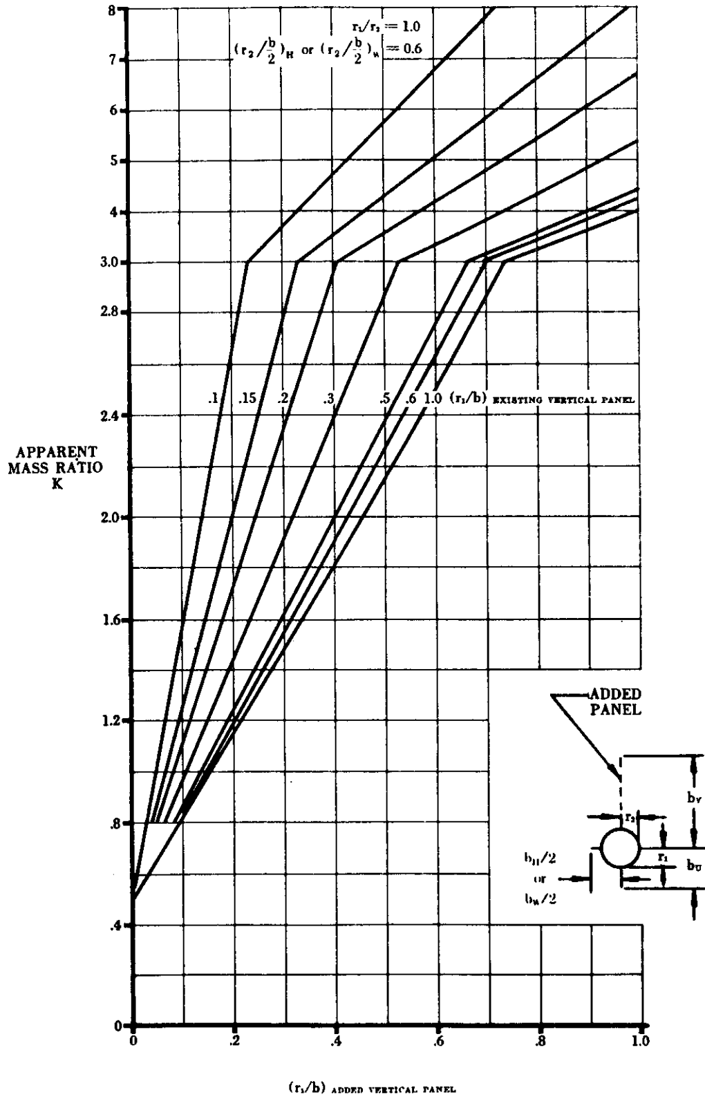
FIGURE 5.3.1.1-25e APPARENT MASS FACTORS (CONTD)
