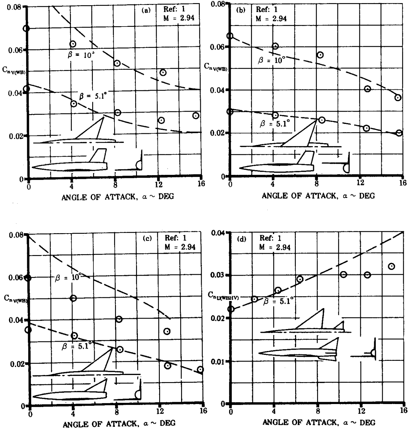
FIGURE 5.6.3.2-4 COMPARISON OF EXPERIMENTAL AND CALCULATED YAWING-MOMENT COEFFICIENT INCREMENTS DUE TO ADDING A VERTICAL TAIL TO A WING-BODY
