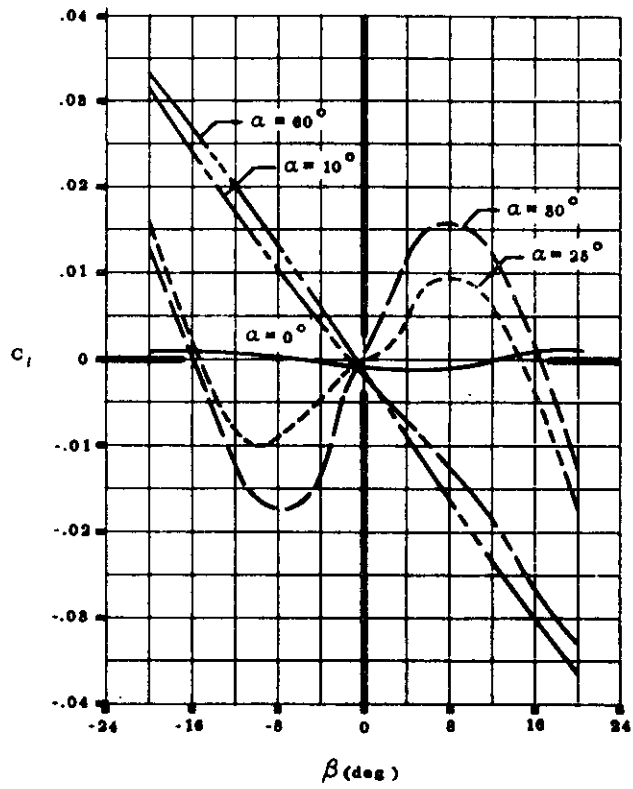
FIGURE 5.1.2.2-5 VARIATIONS OF ROLLING MOMENT WITH SIDESLIP FOR A DELTA WING AT LOW SPEEDS, ZERO DIHEDRAL. (REF. 1).
