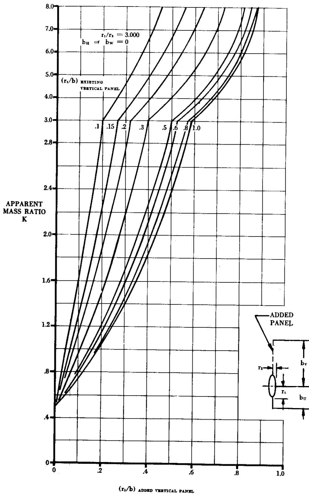
FIGURE 5.3.1.1-25ii APPARENT MASS FACTORS (CONTD)
