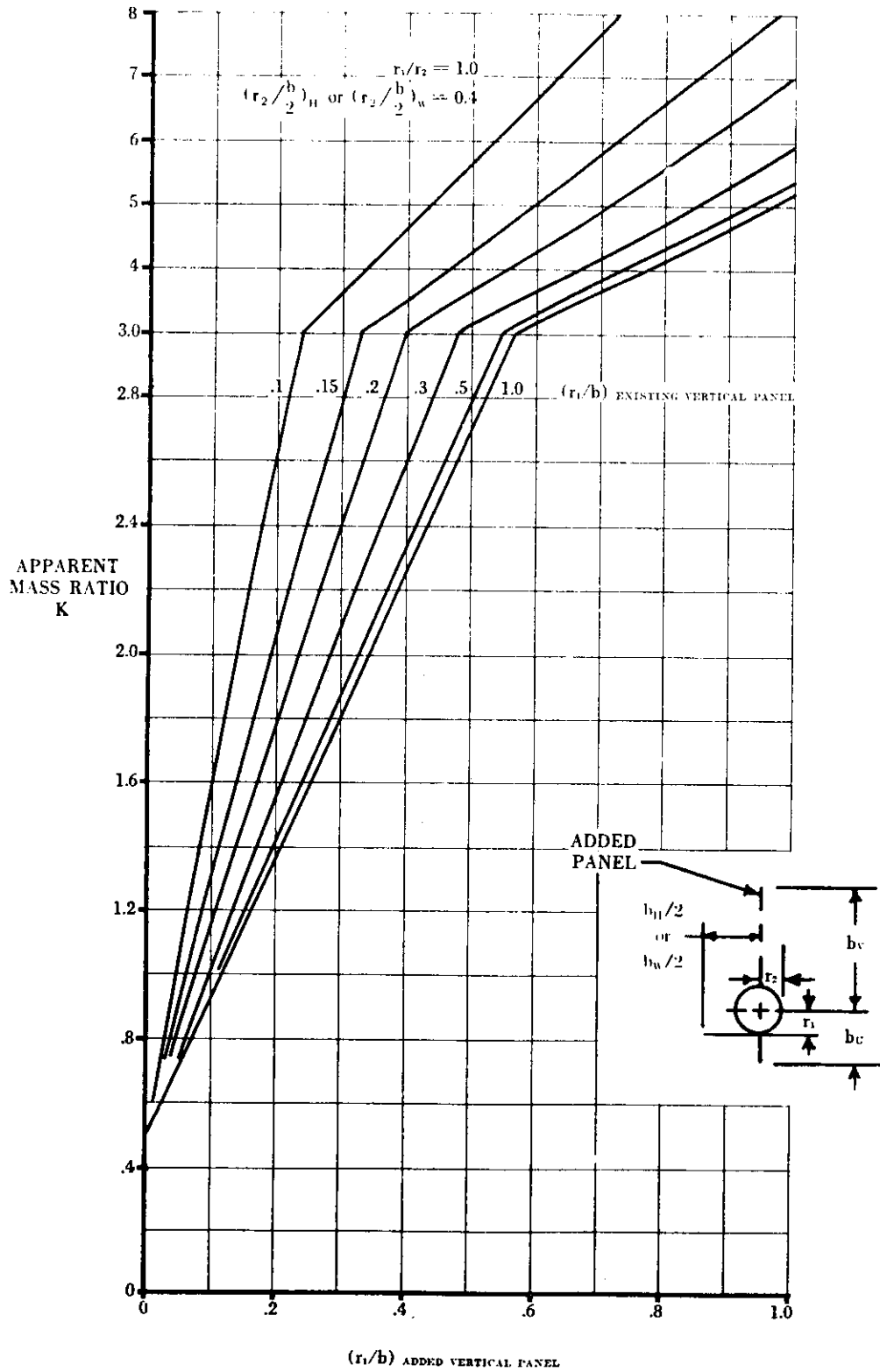
FIGURE 5.3.1.1-25n APPARENT MASS FACTORS (CONTD)
