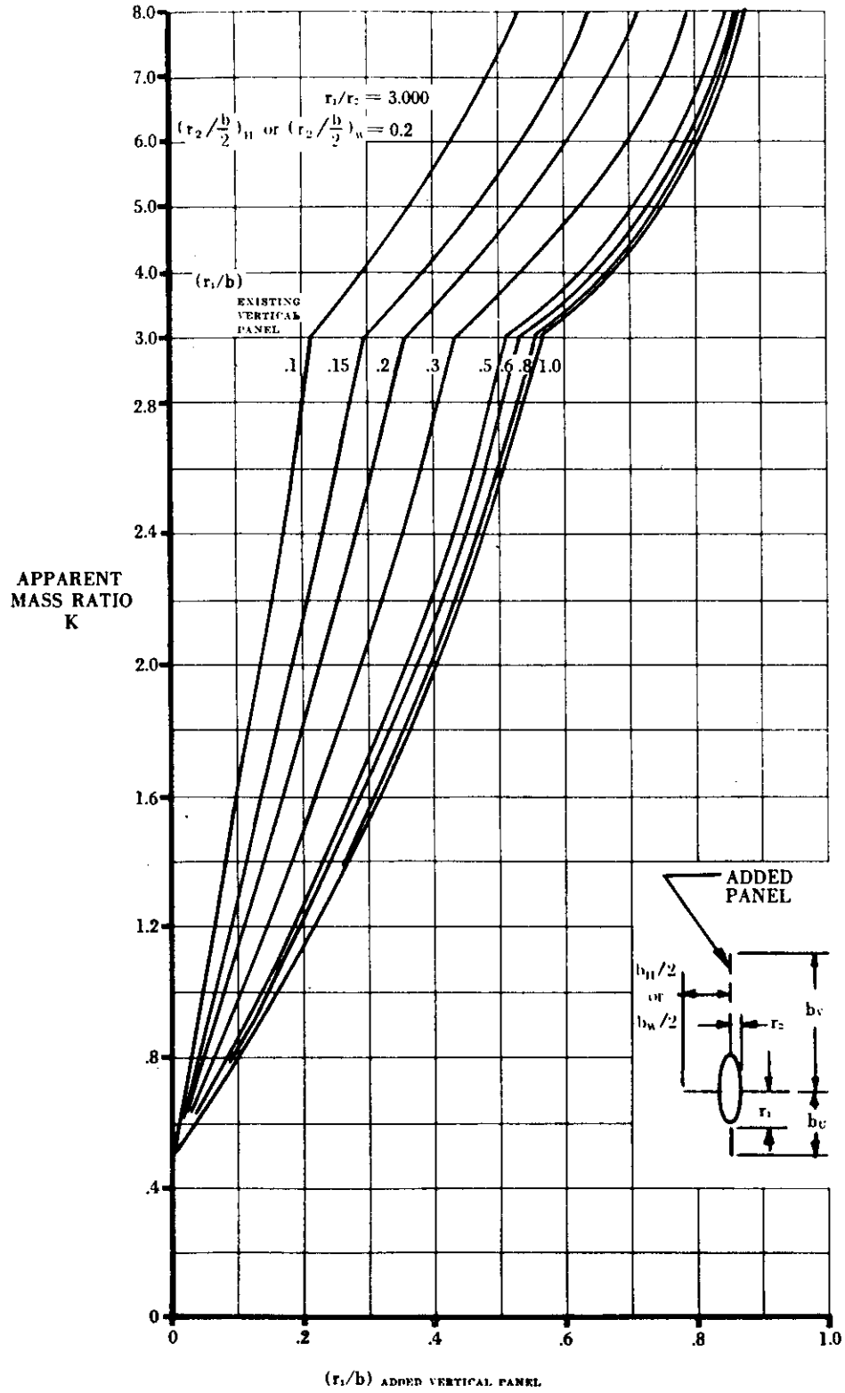
FIGURE 5.3.1.1-25kk APPARENT MASS FACTORS (CONTD)
