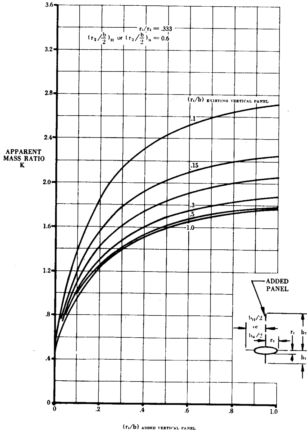
FIGURE 5.3.1.1-25u APPARENT MASS FACTORS (CONTD)
